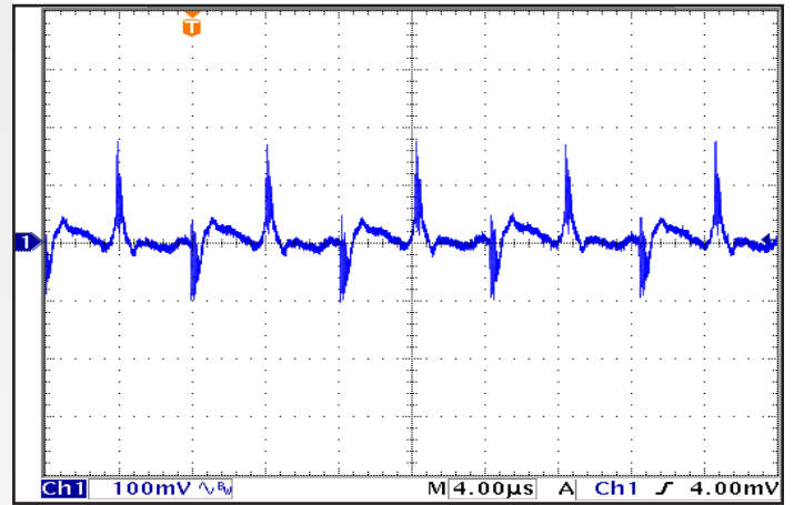
Figure 10: Output Voltage Ripple , V_{out} , at nominal input voltage and rated load current (100 mV/div). Load capacitance: 1 \mu F ceramic and 470 \mu F electrolytic capacitors. Bandwidth: 20 MHz. Timescale: 4.00 \mu s/div. See Figure 13.
