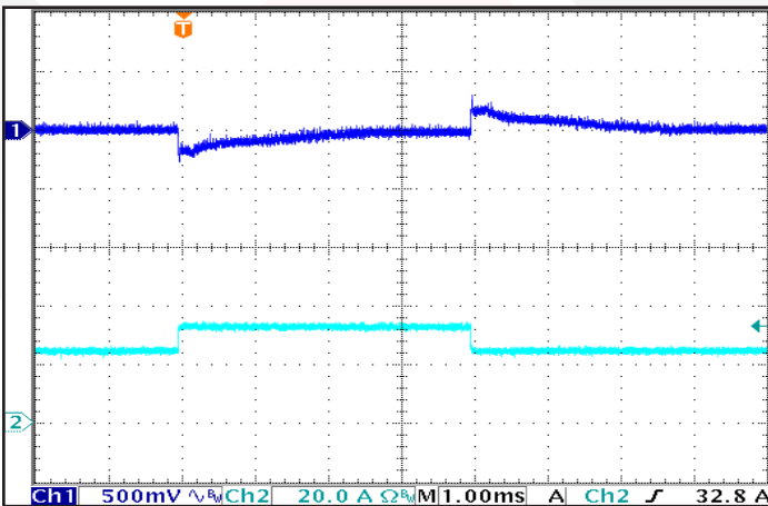
Figure 11: Output Voltage Response to Step-Change in Load Current , (50%-75%-50% of I_{out(max)} ; di/dt = 5 A/ \mu s). Load capacitance: 1 \mu F ceramic and 470 \mu F electrolytic capacitors. Ch 1: \Delta V_{out} (0.5 V/div); Ch 2: I_{out} (20 A/div). Timescale: 1.00ms/div.
