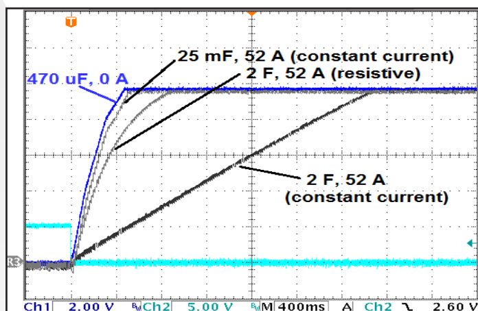
Figure 16: Hi-Cap Option Startup Waveform , input voltage pre-applied. Ch1: V_{out} , 470μF, no load (2V/div); Ref1: 25mF, 52A CC load; Ref2: 2F, 52A CR load; Ref3: 2F, 52A CC load; Ch2: ON/OFF Pin (5V/div). Constant-current loads and large capacitances may slow the startup ramp. Timescale: 400ms/div.
